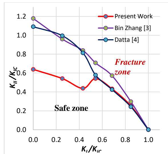
Fig.7 Normalized prediction of the mixed mode fracture criteria of SLGS.
