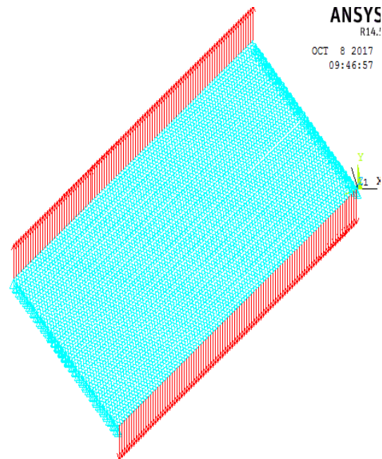
Fig.3 Finite element model of a typical Arcan specimen with 45^\circ .
