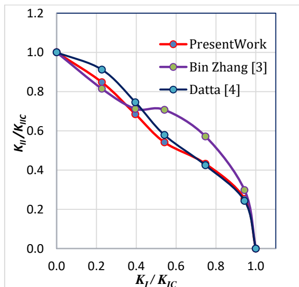
Fig.6 Normalized mixed-mode fracture envelope and predictions of the mixed-mode fracture criteria with a crack length of 25 cells.
