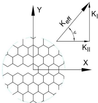
Fig.2 Model of the mixed-mode loading.
